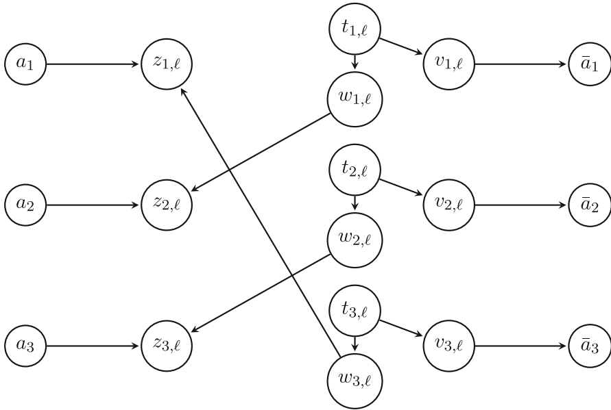
Fig. 4 Dominance relation \triangleright for clause \{u_1, u_2, u_3\}
