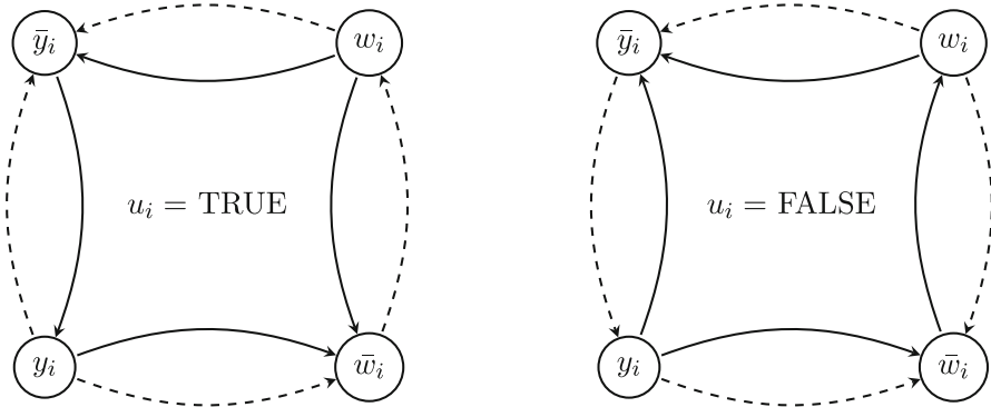
Fig. 2 Value of the variable u_i
